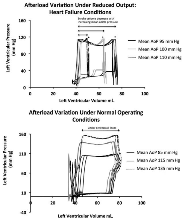
FIG. 4. PV loops with varying afterloads in heart failure and normal conditions. A: PV loops with 95, 100, and 110 mm Hg mean AoPs, corresponding to systolic pressures of 111, 112, and 114 mm Hg respectively. B: PV loops with 85, 115, and 135 mm Hg mean AoPs. Notice the difference in loop trends over the varying afterloads. Stroke volume (loop width) decreases with increased afterload whereas in normal operating conditions stroke volume remains the same over varying afterloads. Normal condition pressure volume loops (Crosby et al., 2014). In heart failure conditions, PV loops with a mean AoP of up to 135 mm Hg (as was tested under normal conditions) was not achievable because flow through the system would cease at higher AoPs.
